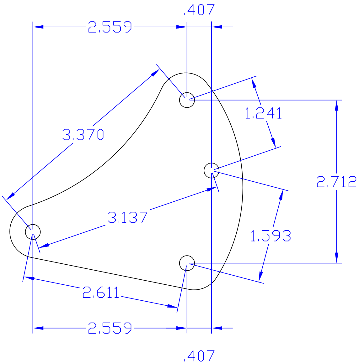
ADAPTER PLATE FOR FH012AA \frac{1}{4} " ALUMINUM
